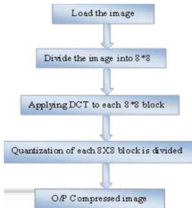
Fig. 1: DCT Image Compression Process
